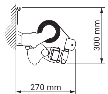
wall installation
