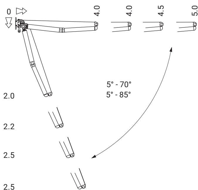
tilt angle
