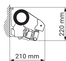
wall installation
