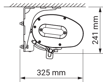
ceiling installation
